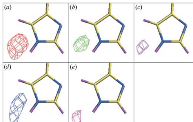
Figure 17 Positive neutron F_o - F_c maps for His51 (all at 2.5\sigma ) at various resolutions (calculated from the model with no D atoms included). (a) 2.2 Å resolution; (b) 2.5 Å resolution; (c) 2.75 Å resolution; (d) 3.0 Å resolution; (e) 3.25 Å resolution.
