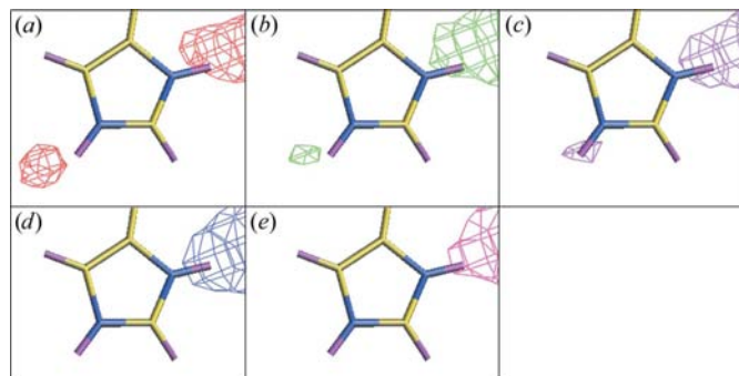
Figure 18 Positive neutron F_o - F_c maps for His180 (all at 2.5\sigma ) at various resolutions (calculated from the model with no D atoms included). (a) 2.2 Å resolution; (b) 2.5 Å resolution; (c) 2.75 Å resolution; (d) 3.0 Å resolution; (e) 3.25 Å resolution.
