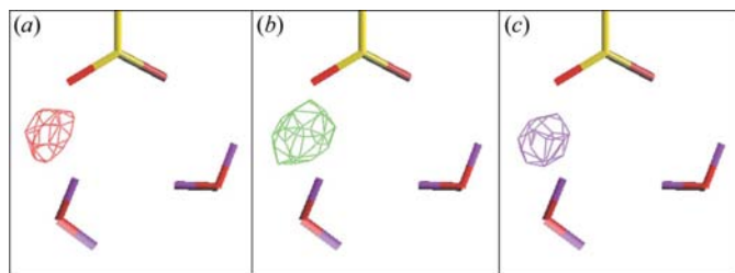
Figure 15 Positive neutron F_o - F_c maps for Asp82 (all at 2.5\sigma ) at various resolutions (calculated from the model with no D atoms included). (a) 2.2 Å resolution; (b) 2.5 Å resolution; (c) 2.75 Å resolution.
