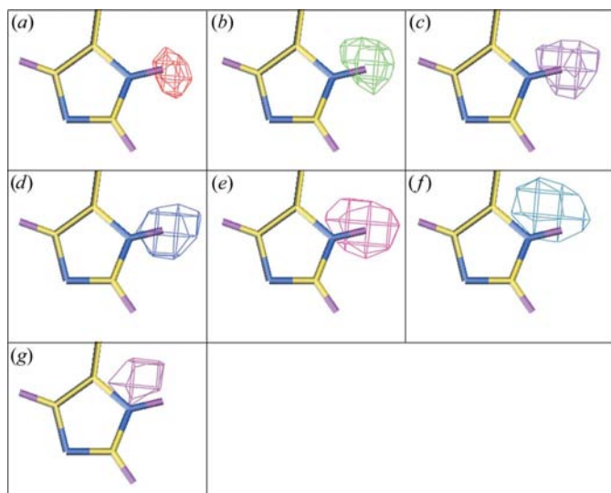
Figure 16 Positive neutron F_o - F_c maps for His24 (all at 2.5\sigma ) at various resolutions (calculated from the model with no D atoms included). (a) 2.2 Å resolution; (b) 2.5 Å resolution; (c) 2.75 Å resolution; (d) 3.0 Å resolution; (e) 3.25 Å resolution; (f) 3.5 Å resolution; (g) 3.75 Å resolution.
